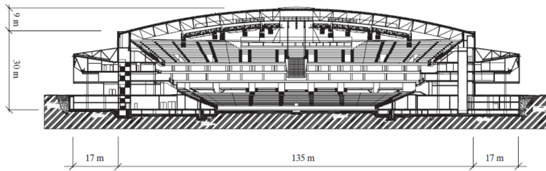
Fig. 1: Cross-section of the Arena
