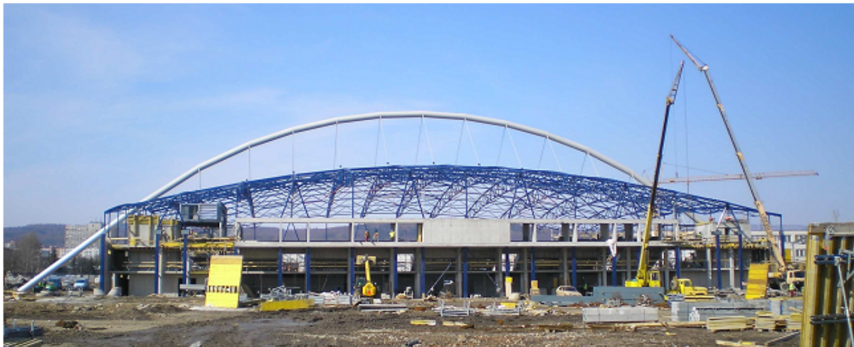
Fig. 5: Roof steel structure after assembly
