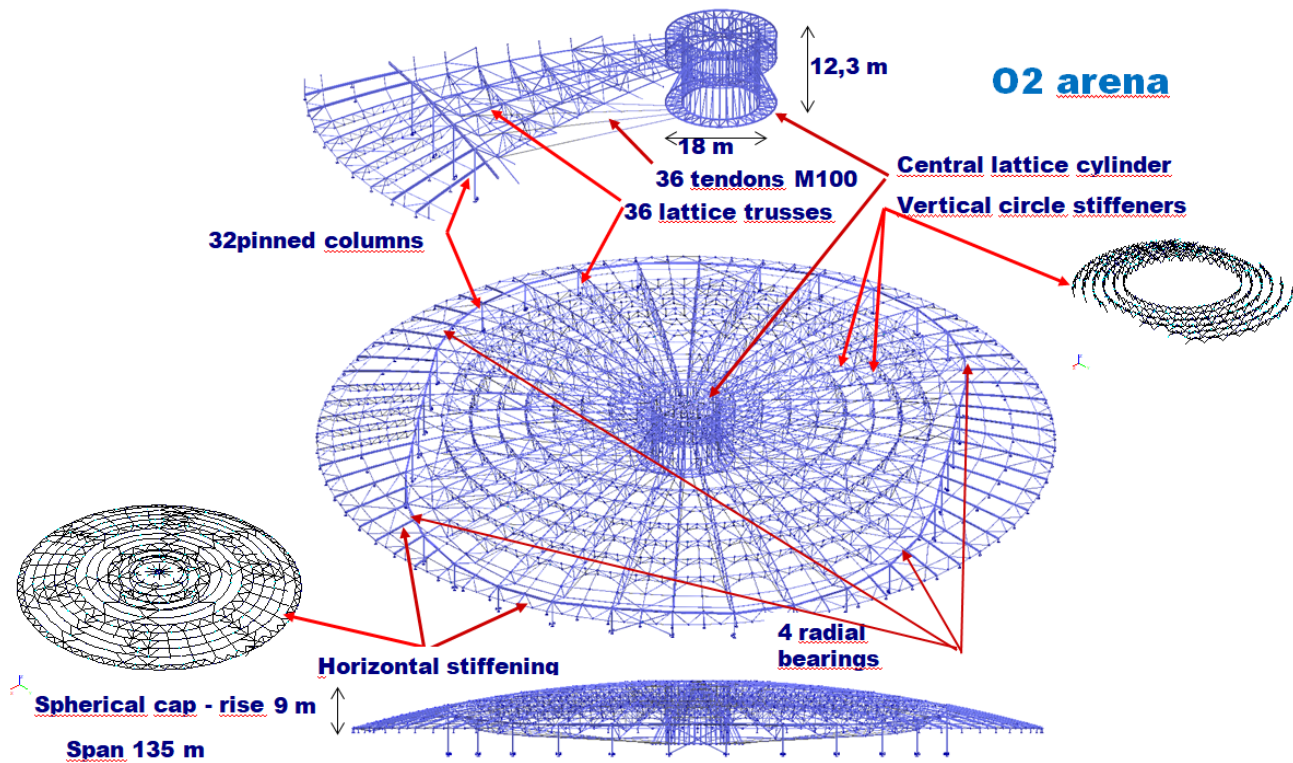
Fig. 2: Static model of the Arena
