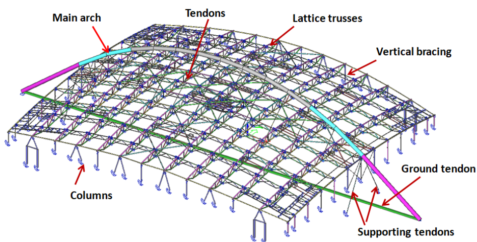
Fig. 6: Steel structure – static spatial model
