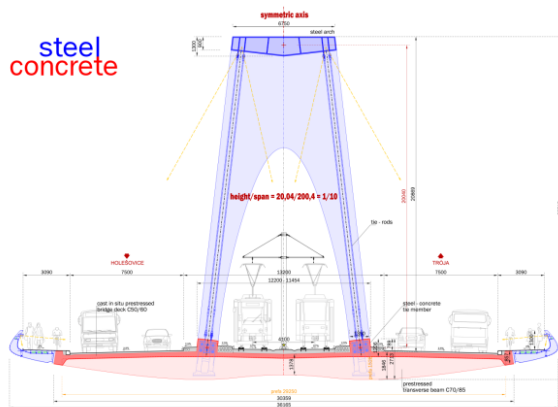
Fig. 14: Cross-section
