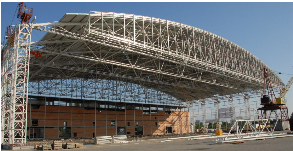
Fig. 9: Hangar Mošnov after lifting of the roof structure
