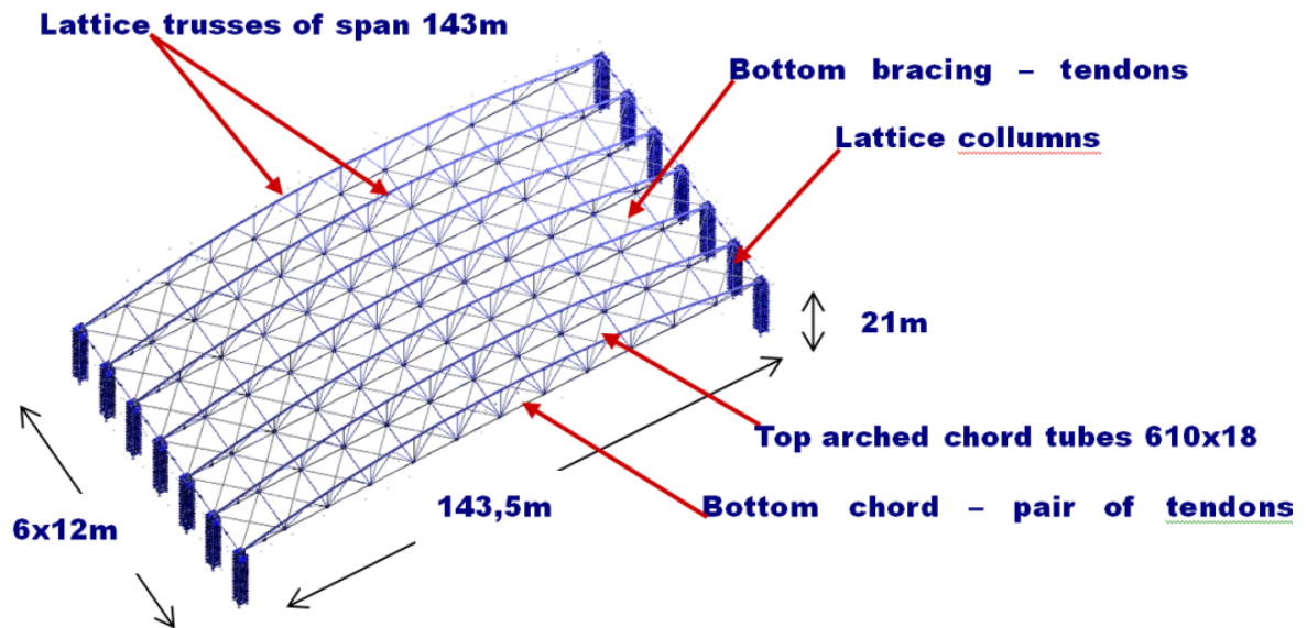
Fig. 10: Steel structure – static spatial model
