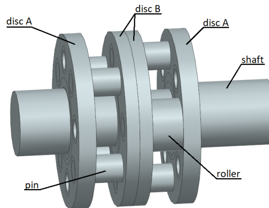
Fig. 1: Turret follower assembly
