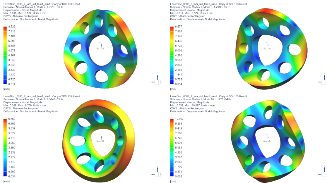
Fig. 3: Hybrid (Forged 50 %) disc mode shapes.
