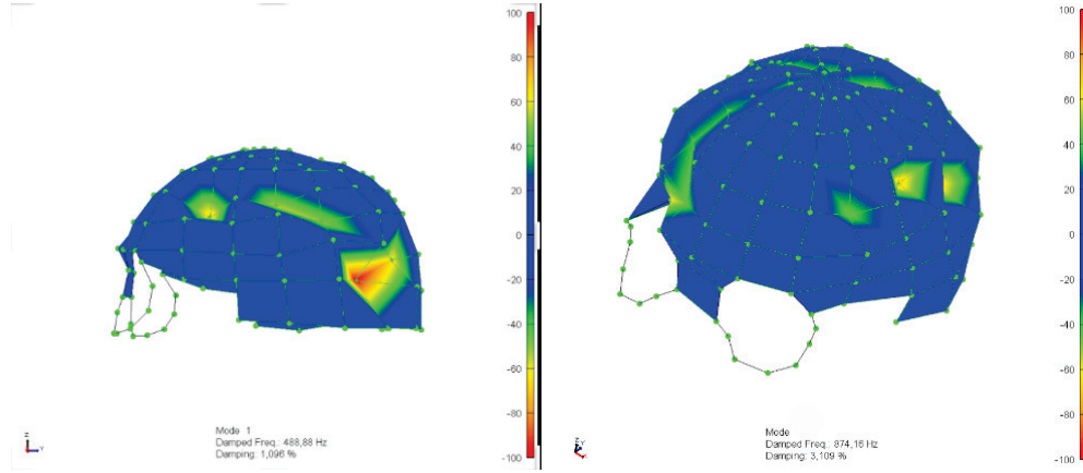
Fig. 5: Modal shapes at 488.8 Hz & 874.1Hz
