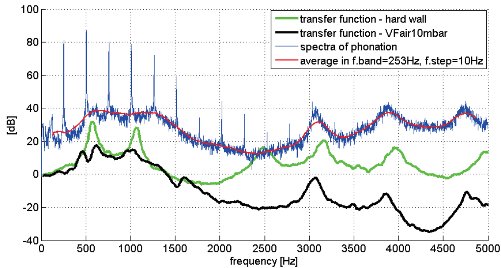
Fig. 4: The volume velocity transfer function measured for the hard wall at the position of the vocal folds and for VF model filled with air; spectra of the acoustic signal measured 20 cm from the lips during self-oscillation of the VF model filled with air.
