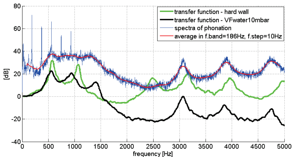
Fig. 3: The volume velocity transfer function measured for the hard wall at the position of the vocal folds and for VF model filled with water; spectra of the acoustic signal measured 20 cm from the lips during self-oscillation of the VF model filled with water.
