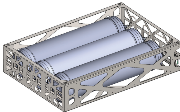
Fig. 2: Bundle of pressure cylinders.
