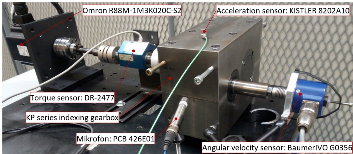
Fig. 3: Test device.
